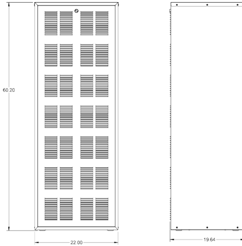
AM-602220-MTR (32RU)
