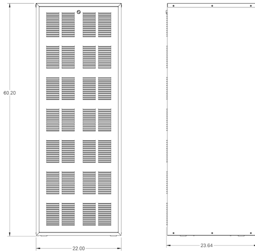
AM-602224-MTR (32RU)
