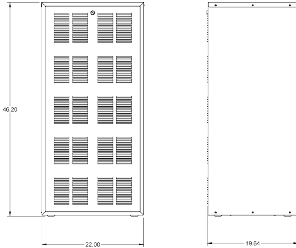
AM-462224-MTR (24RU)
