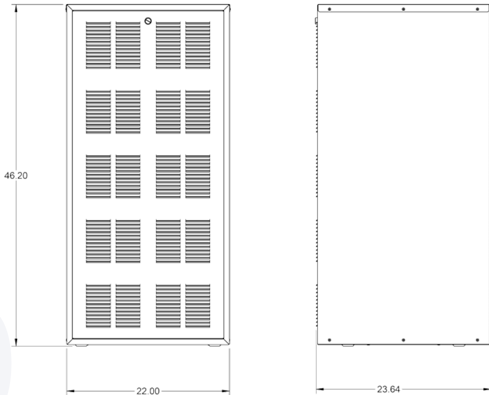
AM-462224-MTR (24RU)
