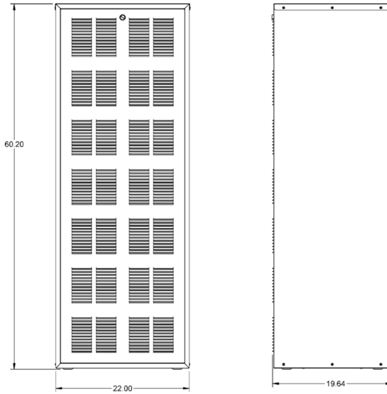
AM-602220-MTR (32RU)
